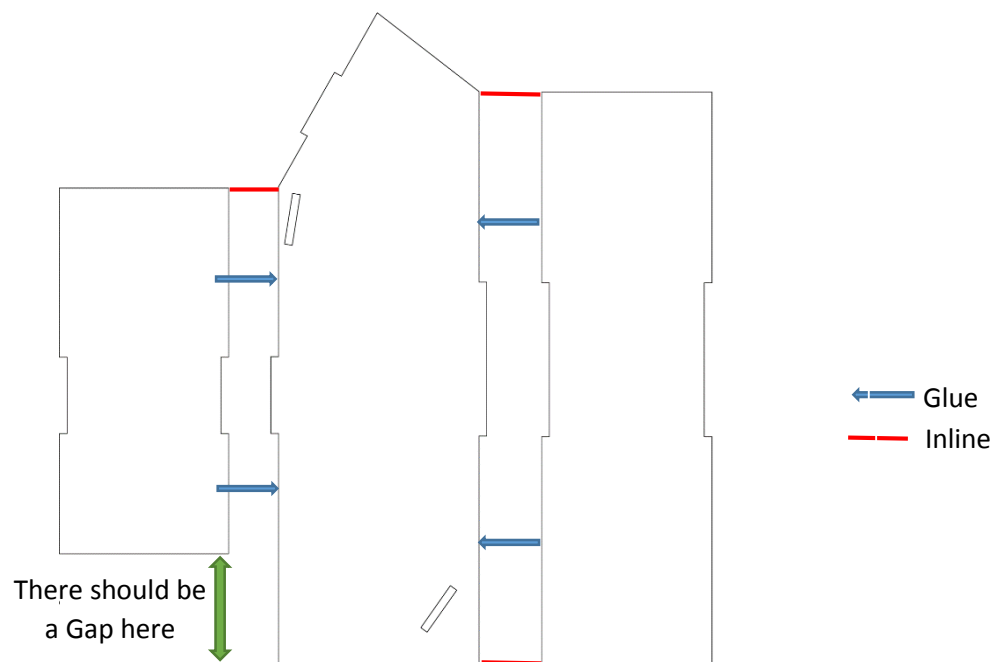
Figure 2 Assembling the front and back sections of the periscope
